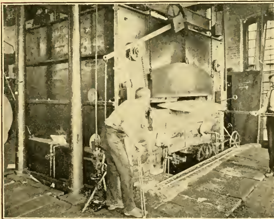
TEMPERING CIRCULAR SAWS
